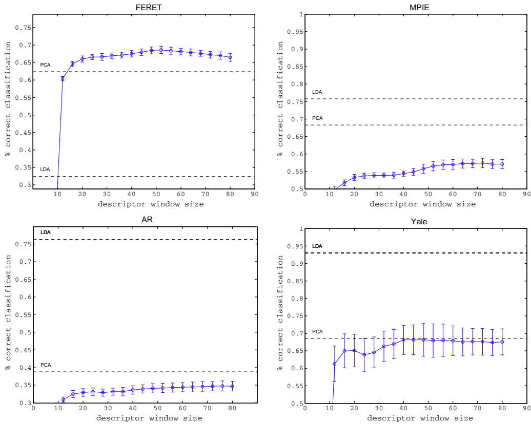
Fig. 3. Recognition rates (with standard deviations) using HOG features extracted from facial landmarks (10 runs with random training-test distribution of samples). The dashed lines show the recognition results using standard PCA and LDA (we use the number of bases that gave best results in the test set).
