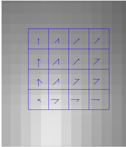
Fig. 1. Example HOG descriptors, patch size=8 × 8. Each cell of the patch shows the orientation of the gradients.
