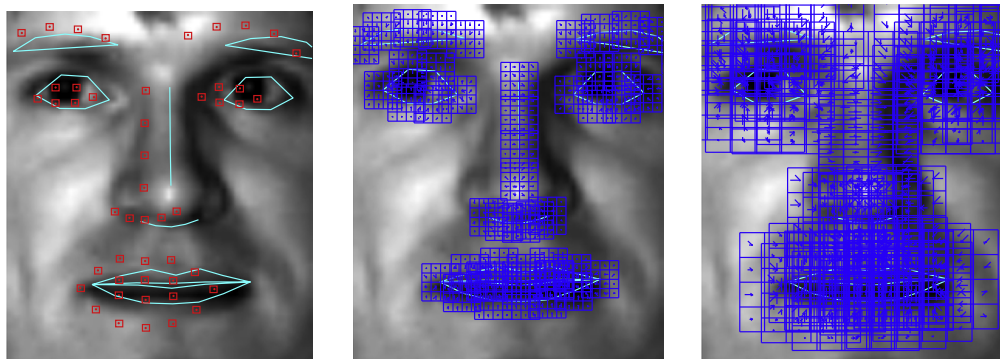
Fig. 2. Left: Initialized landmarks (red boxes) and result for the AAM fitting in an image from the Yale database. Center: extracted HOG descriptors, patch size = 24 × 24. Right: extracted HOG descriptors, patch size = 64 × 64. (For interpretation of the references to color in this figure legend, the reader is referred to the web version of this article.)
